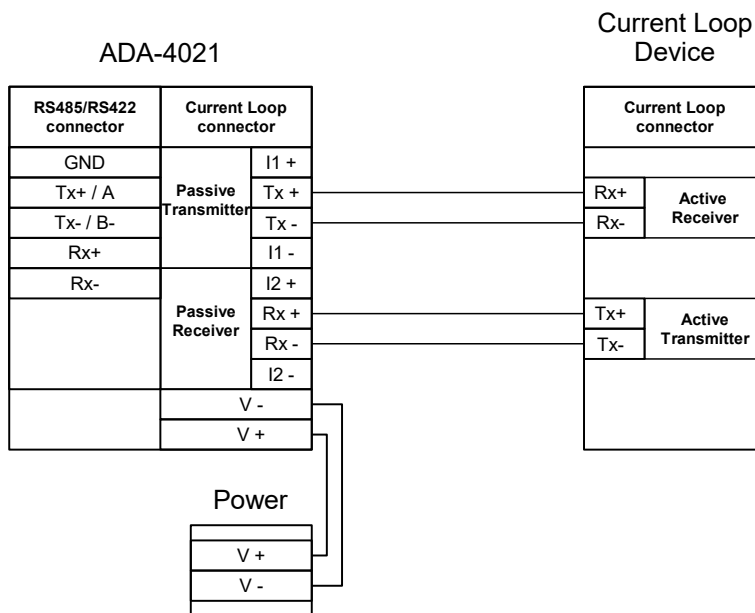
Fig 9. Example connection of device with active transmitter and active receiver to ADA-4021
