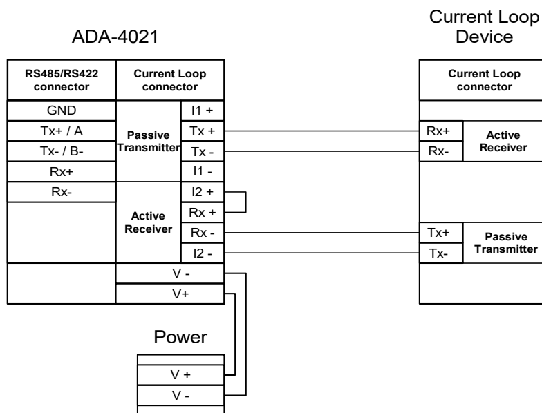
Fig 11. Example connection of device with passive transmitter and active receiver to ADA-4021
