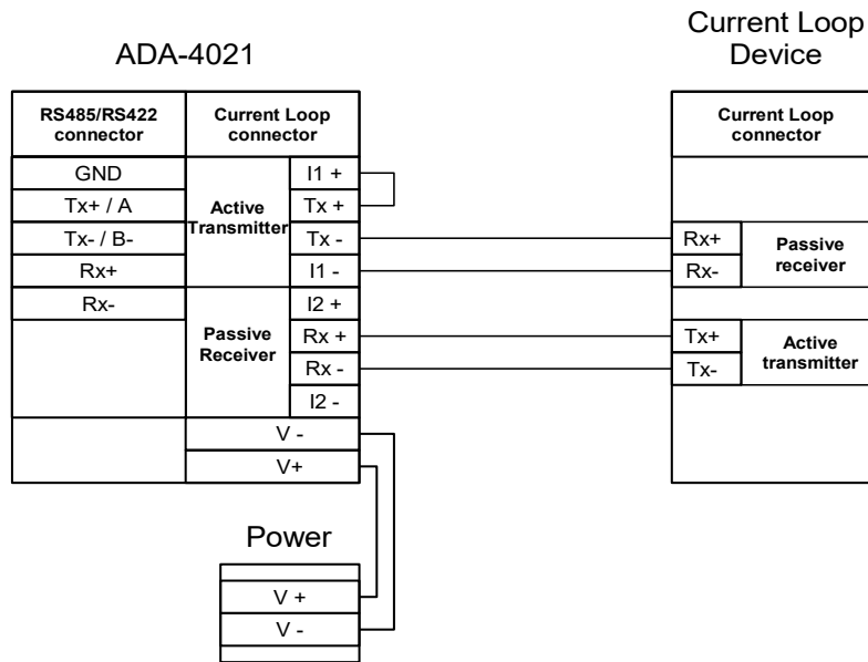
Fig 10. Example connection of device with active transmitter and passive receiver to ADA-4021
